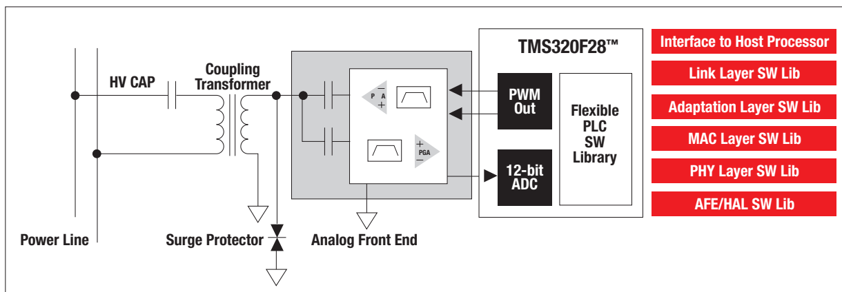
▲ Figure 2. TI's narrowband PLC solution
